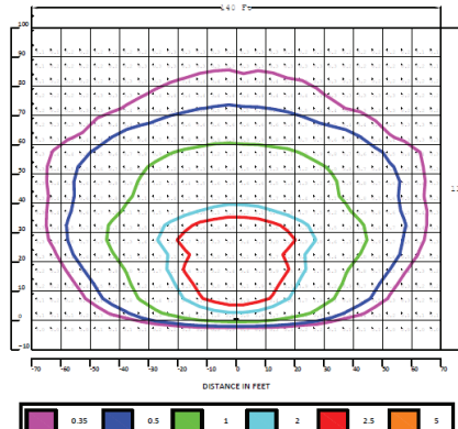
LFLJ17LUT76 @ 40 Ft High; Tilt Angle = 45° (ISOFOOTCANDLES)
