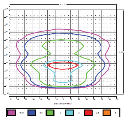
LFLJ12LUT76 @ 40 Ft High; Tilt Angle = 45° (ISOFOOTCANDLES)
