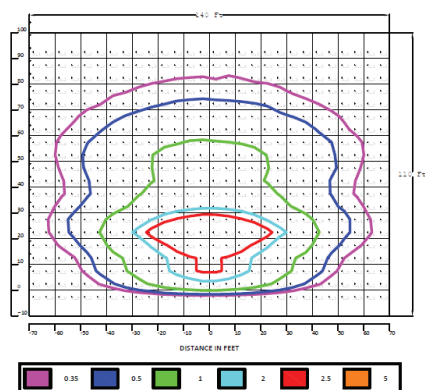
LFLJ13LUT76 @ 40 Ft High; Tilt Angle = 45° (ISOFOOTCANDLES)
