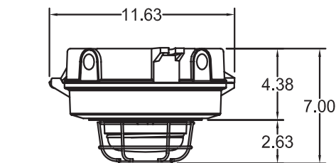
Ceiling mount with threaded glass globe and guard.
