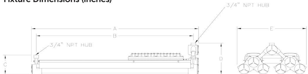
Fixture Dimensions (inches)
